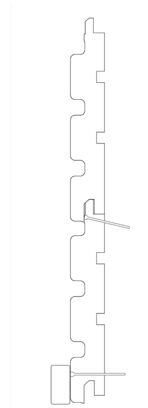
Example of concealed fixing
