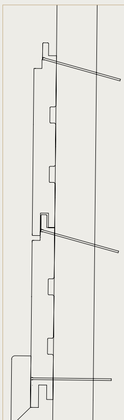
Example of concealed fixing
