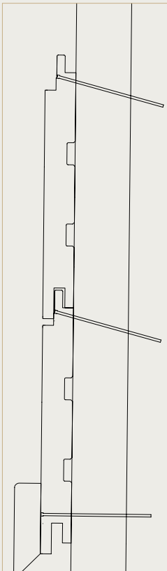
Example of concealed fixing
